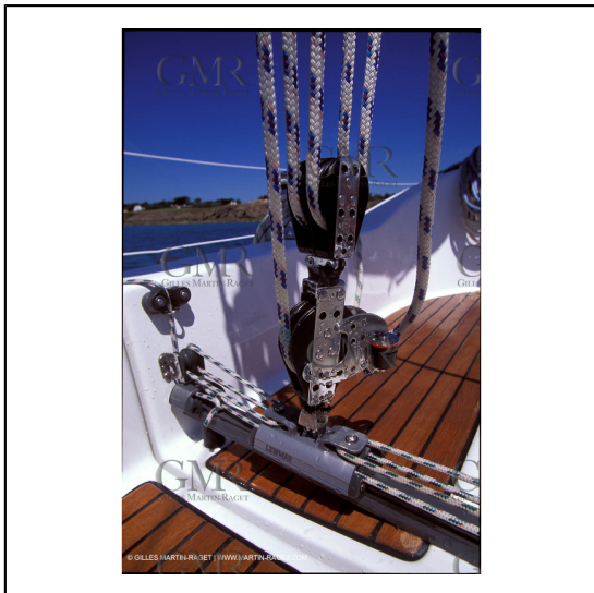
Accastillage***Deck fitting
